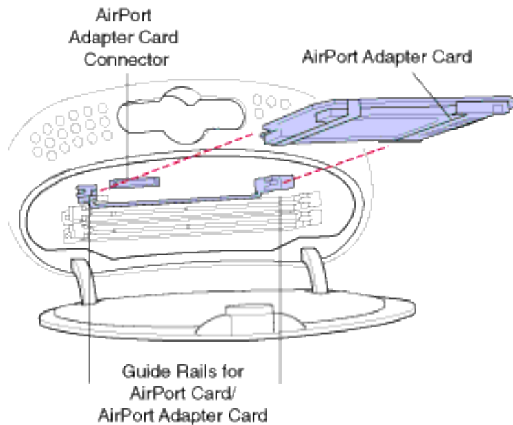
Figure 1 Inserting the AirPort Adapter Card
